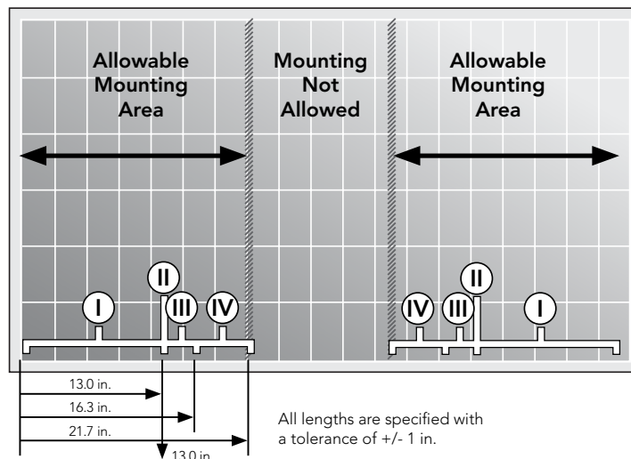
Figure 8: The location of different sections in the allowable mounting area
