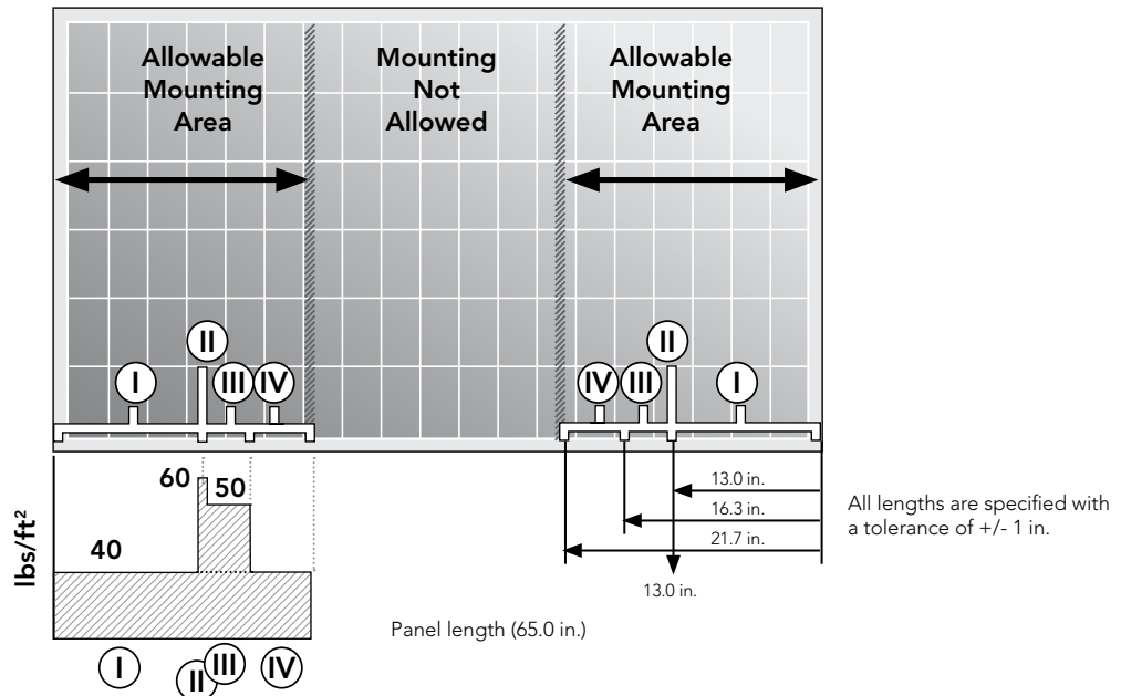
Figure 9: Maximum permissible combined wind and snow loads by rail location
