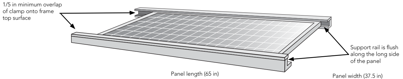
Figure 11: Long-side end mounting
