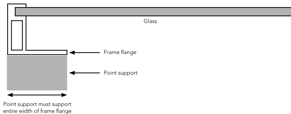
Figure 14: Location of point support in relation to the panel frame
