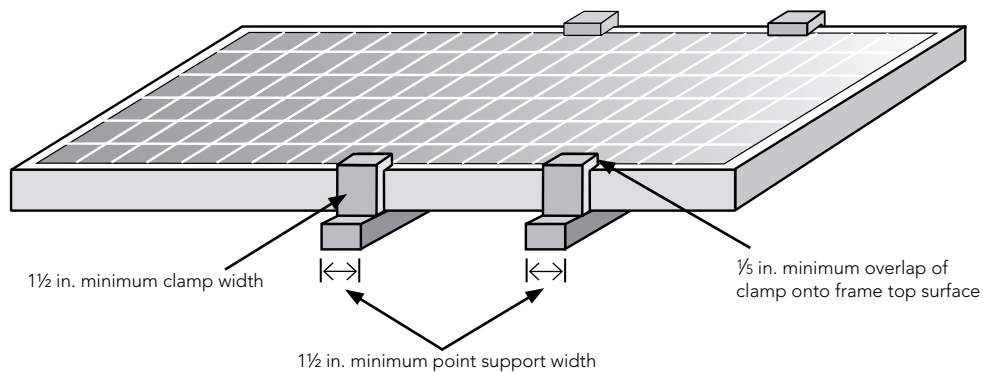
Figure 13: Point support and clamp requirements
