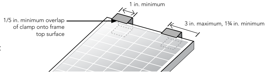
Figure 6: Clamping each panel without rails in direct contact with the panel
