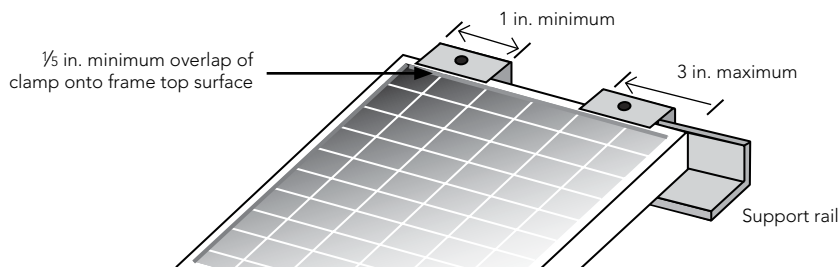
Figure 5: Clamping each panel frame individually
