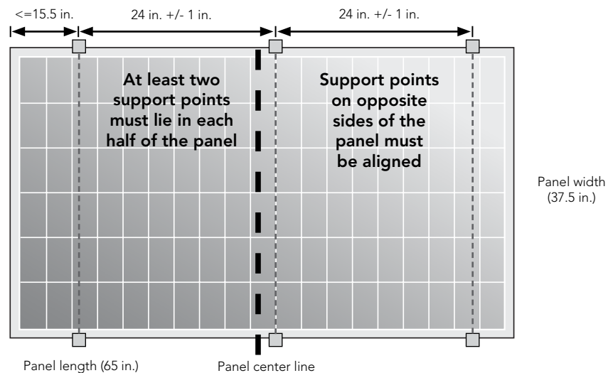
Figure 16: Required support locations for the 6 point option
