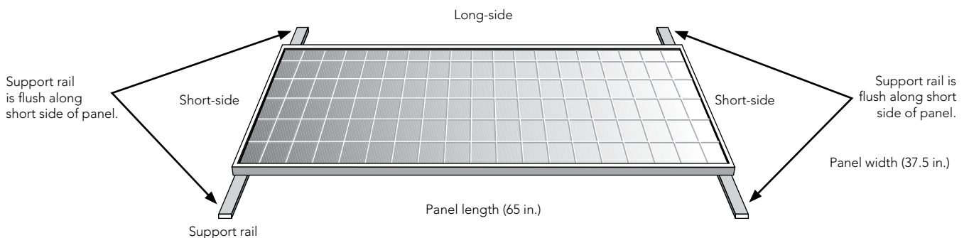
Figure 2: Short-side end mounting
