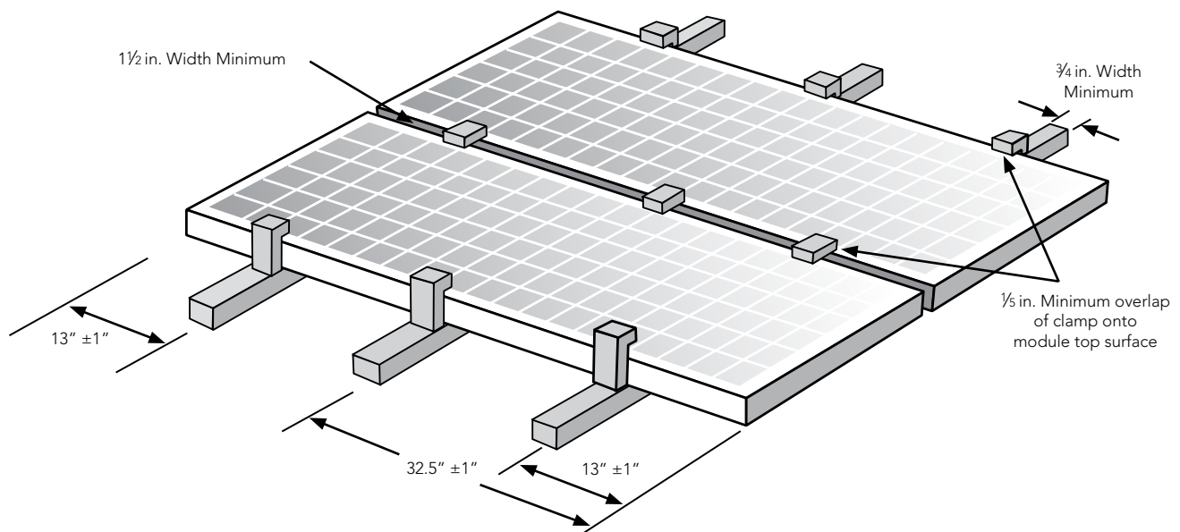
Figure 12: Permissible clamp arrangement for three support rail mounting
