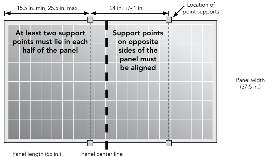
Figure 15: Required support locations for the 4 point option
